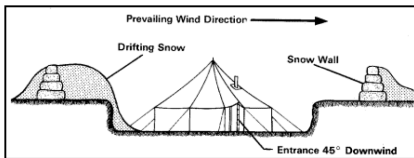
Figure 3-2. Windbreak.
