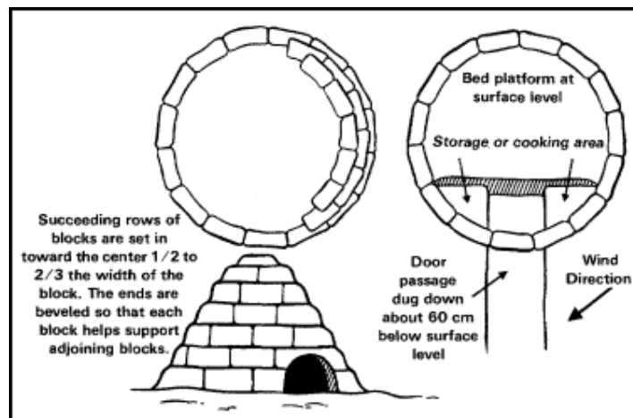
Figure 10-9. Snow house.
