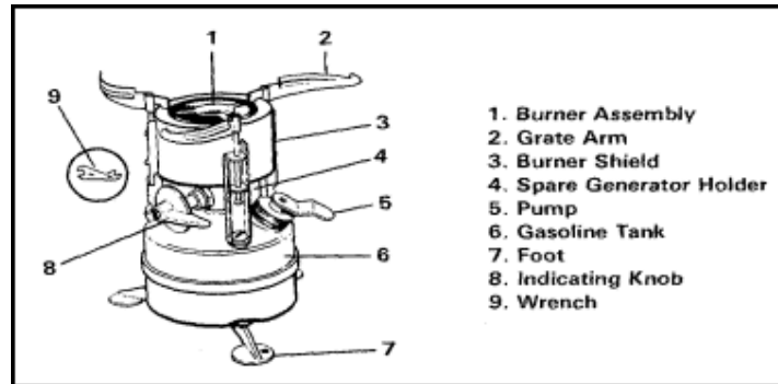
Figure 3-6. Gasoline cooking stove, M1950.
