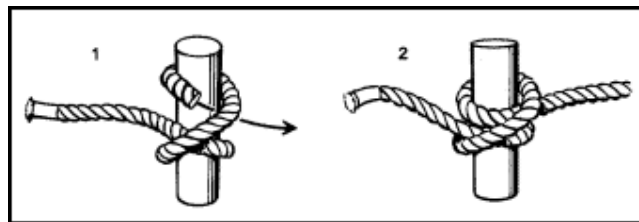
Figure 10-17. Clove hitch.
