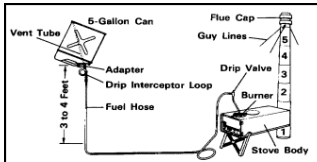
Figure 3-4. Yukon stove.
