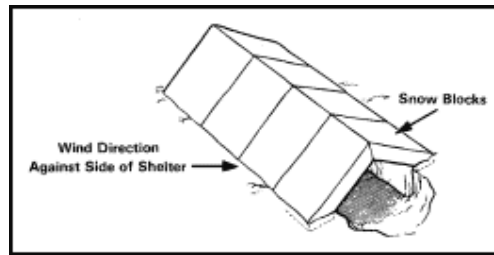
Figure 10-6. Snow trench.
