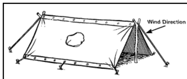
Figure 10-2. Two-man shelter.
