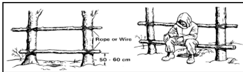
Figure 7-2. Cross-tree type latrine.
