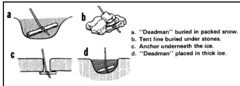
Figure 3-3. Deadmen.
