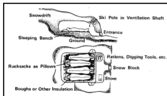
Figure 10-7. Snow cave.
